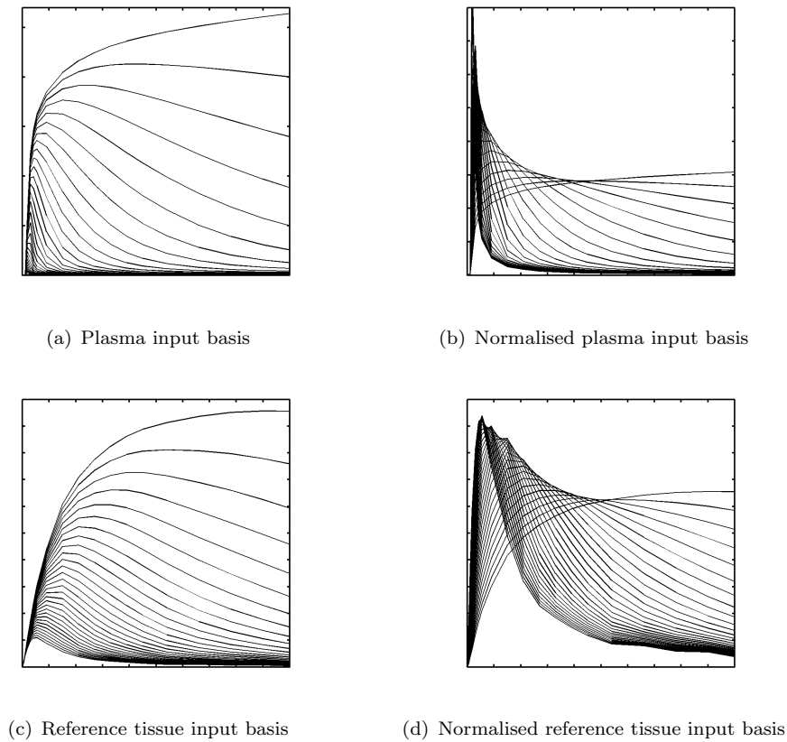
FIGURE 2: Example Dictionaries ( \Psi )
