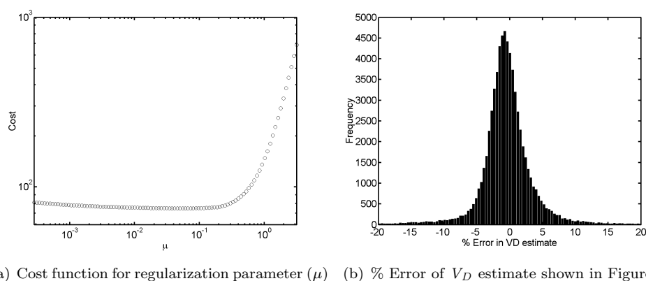
FIGURE 10: 4D Simulation: Cost function and error in V_D estimate.
